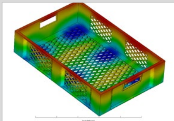
Mould flow analyse
